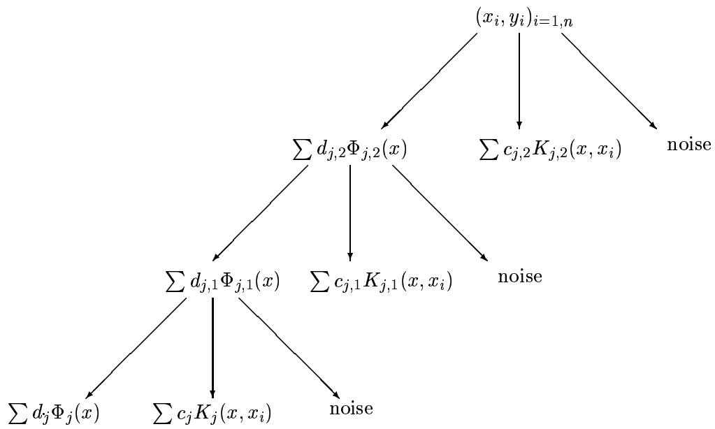
Figure 5: Example of multiscale approximation on 3 levels : the kernel point of view
