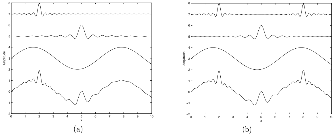
Figure 6: Original functions used for benchmarking in experiment 3. (a) f_1 (b) f_2 . Top : multiscale structure on 3 levels. Bottom : Complete function.
