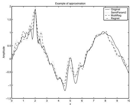
Figure 7: Examples of approximation of f_1 : Original function (Solid), Semiparametric 2 (dotted), Multiscale regularization (dashed), Regularization network (dash-dotted)
