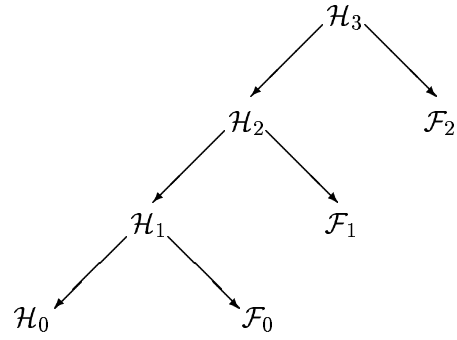
Figure 4: Example of multiscale approximation on 3 levels
