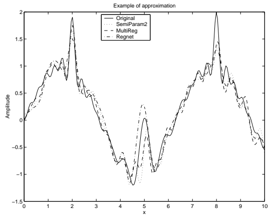
Figure 8: Examples of approximation of f_2 : Original function (Solid), Semiparametric 2 (dotted), Multiscale regularization (dashed), Regularization network (dash-dotted)
