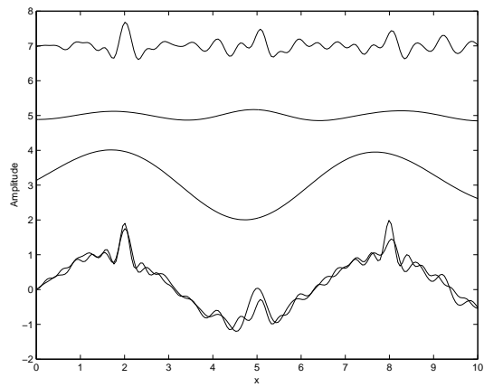
Figure 10: Top : Multiscale structure of a typical prediction of f_1 by multiscale wavelet approximation Bottom : full approximation and true function
