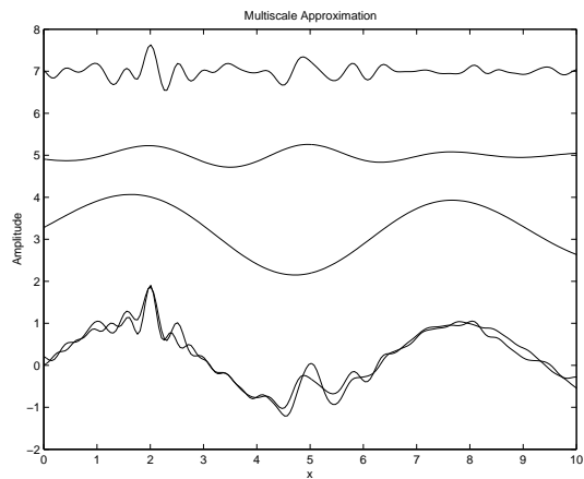
Figure 9: Top : Multiscale structure of a typical prediction of f_1 by multiscale wavelet approximation Bottom : full approximation and true function
