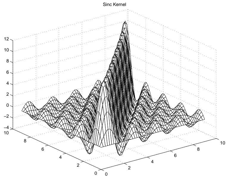
Figure 3: The sinc Kernel.
