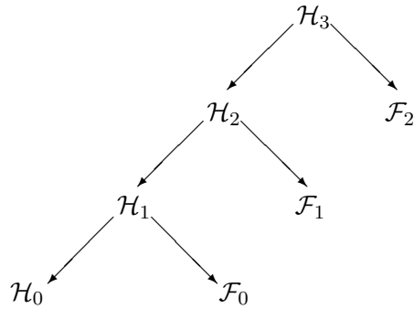
Figure 3: Example of multiscale approximation on 3 levels. Each space \mathcal{H}_j can be decomposed in a trend space \mathcal{H}_{j-1} and a detail space \mathcal{F}_{j-1} . In this case, \mathcal{H}_3 can be considered as the sum of \mathcal{H}_0 , \mathcal{F}_0 , \mathcal{F}_1 and \mathcal{F}_2 .
